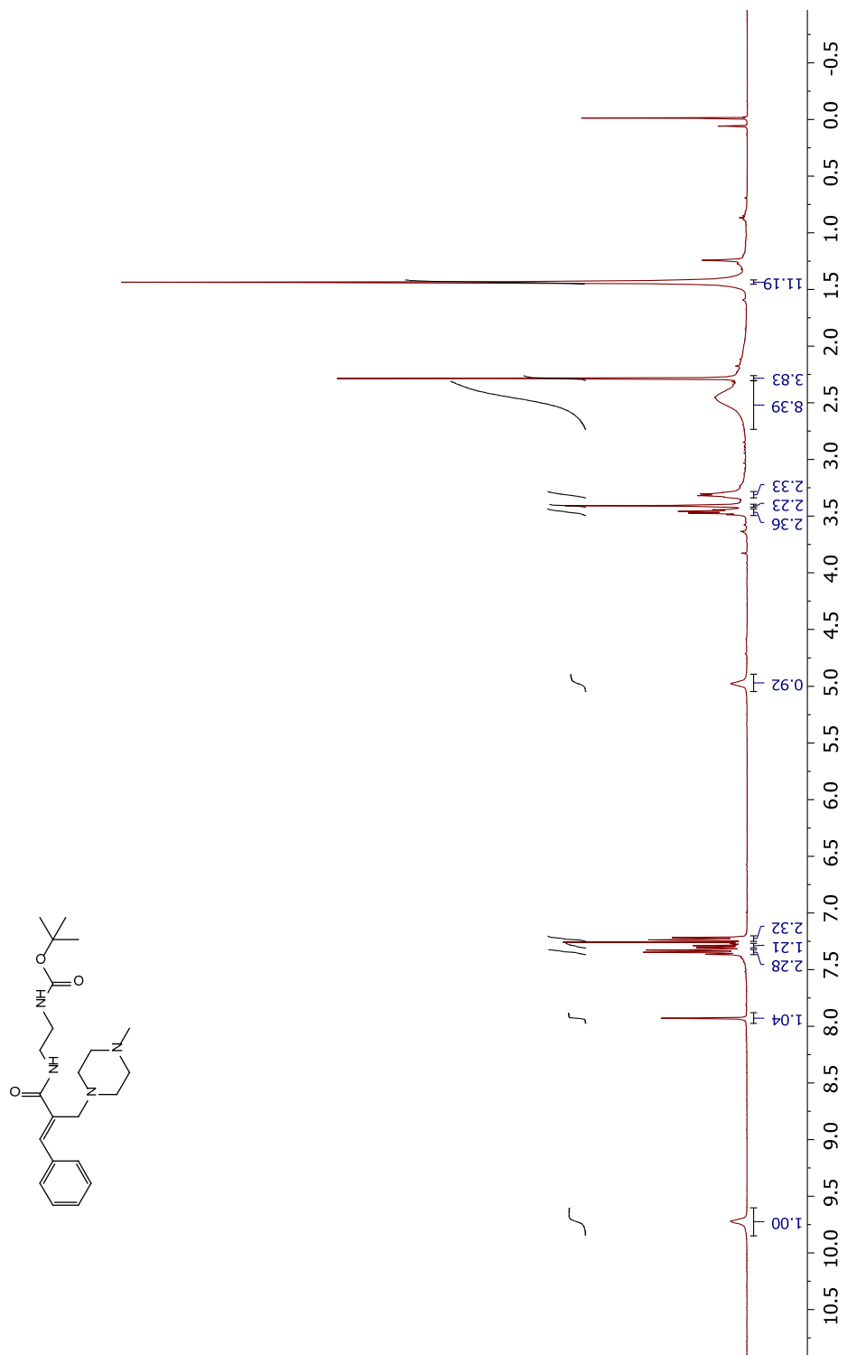
Figure 31. 400 MHz ^1\text{H} NMR of Compound 59 in \text{CDCl}_3
