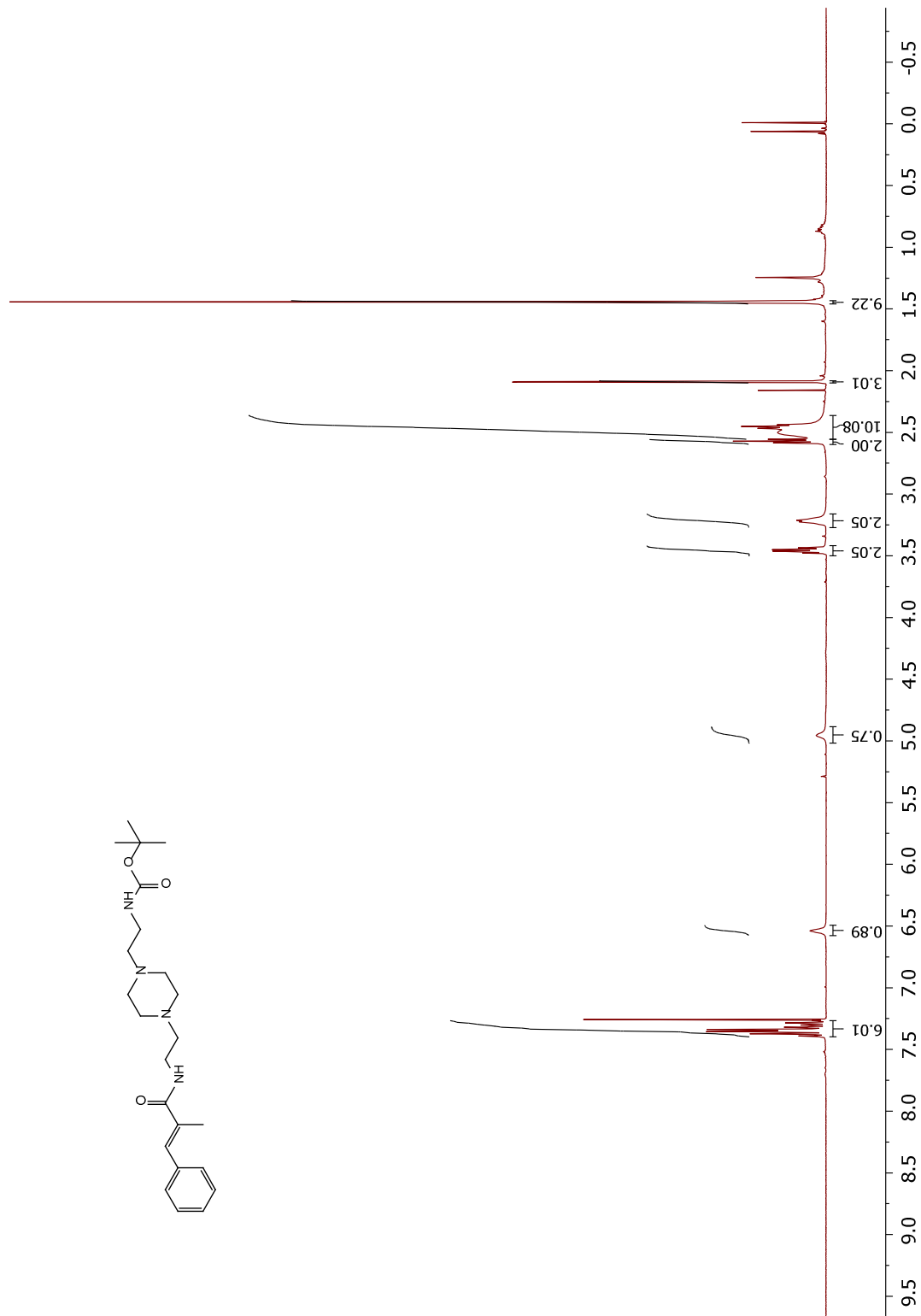
Figure 41. 400 MHz 1 H NMR of Compound 67b in CDCl 3
