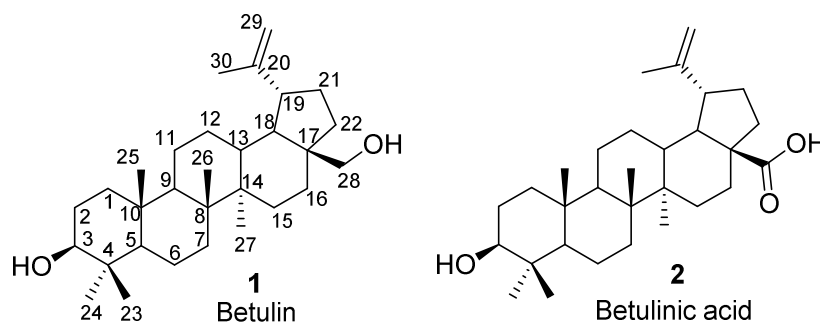
Figure 1. Betulin and Betulinic acid
