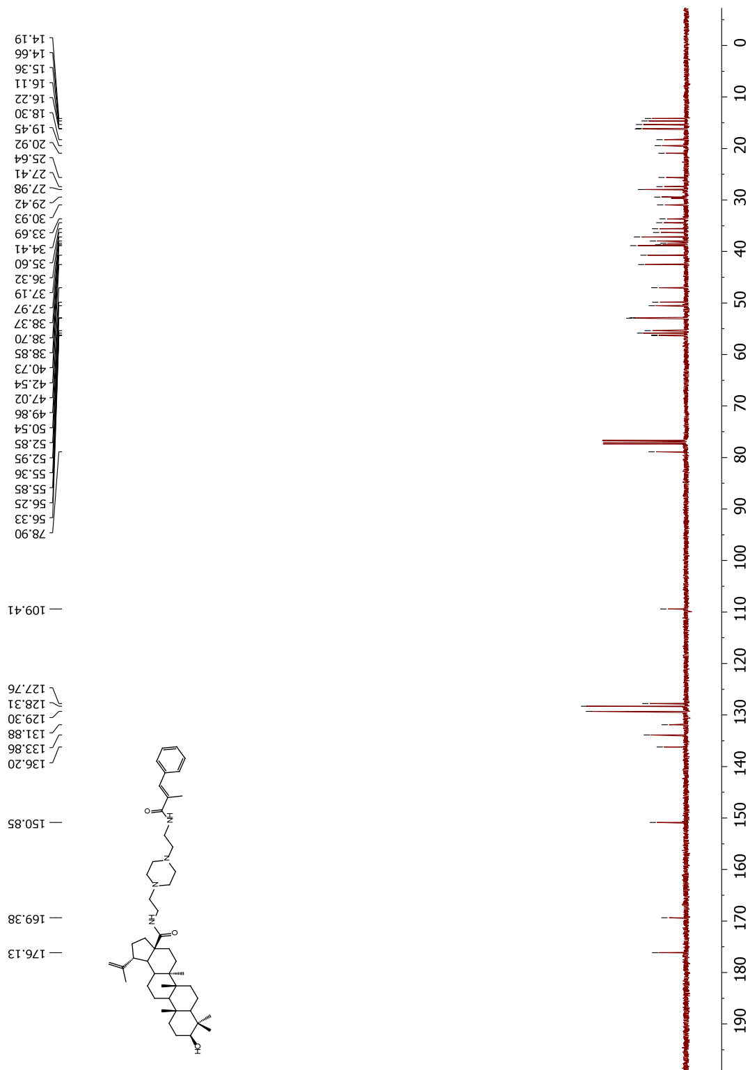
Figure 48. 101 MHz 13 C NMR of Compound 69b in CDCl 3
