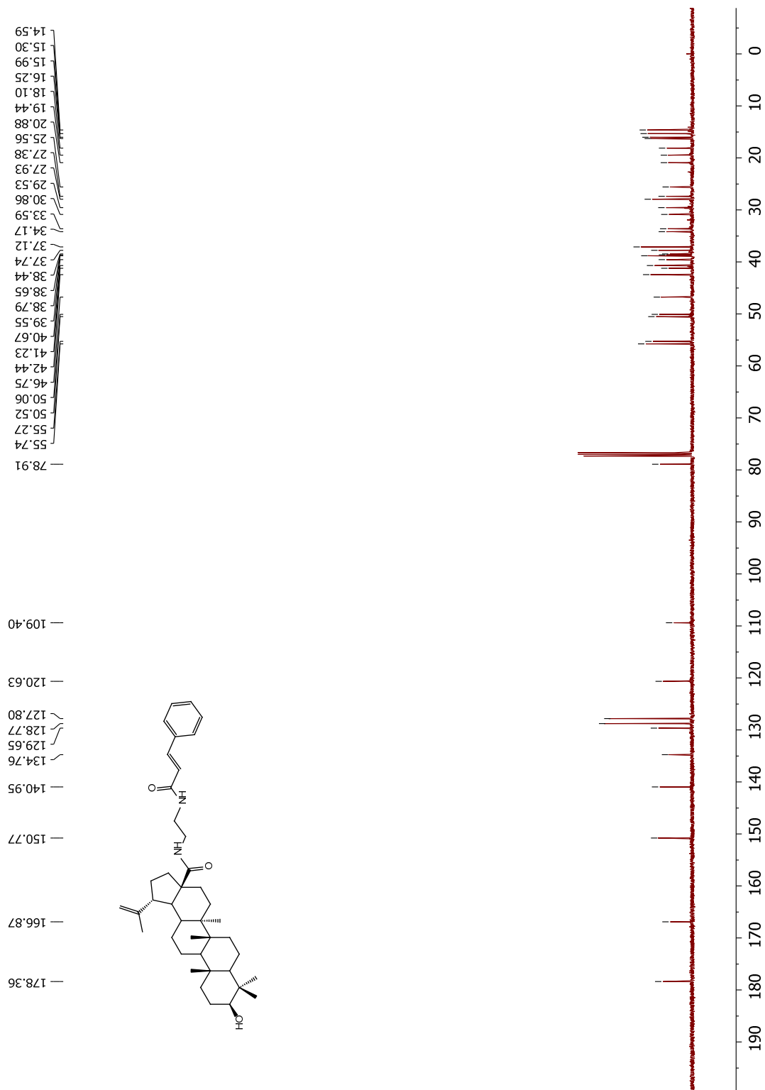
Figure 34. 101 MHz 13 C NMR of Compound 61a in CDCl 3
