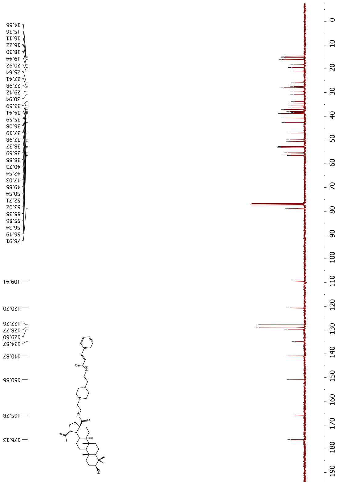
Figure 46. 101 MHz ^{13}\text{C} NMR of Compound 69a in \text{CDCl}_3
