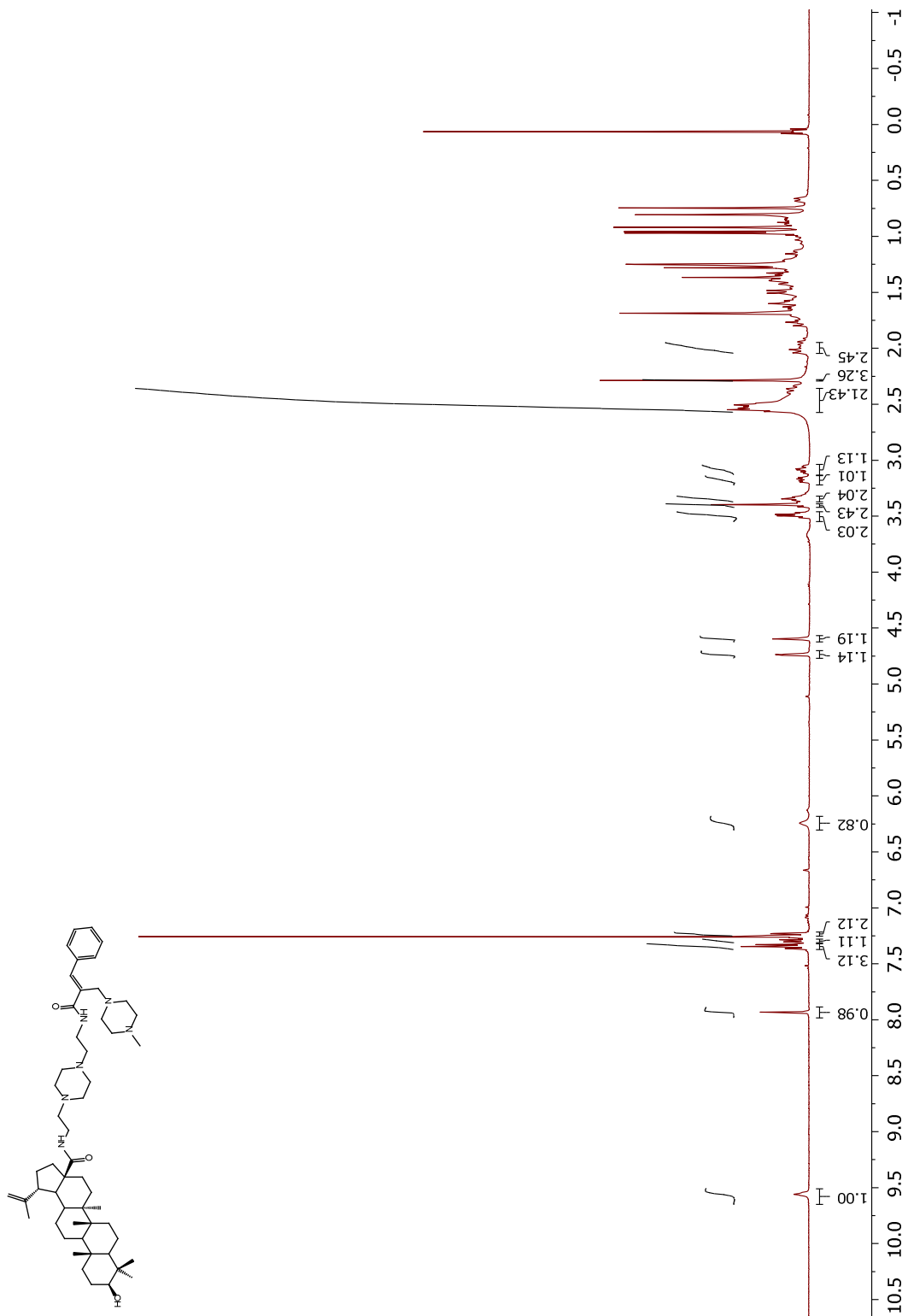
Figure 51. 400 MHz ^1\text{H} NMR of Compound 69d in DMSO- d_6
